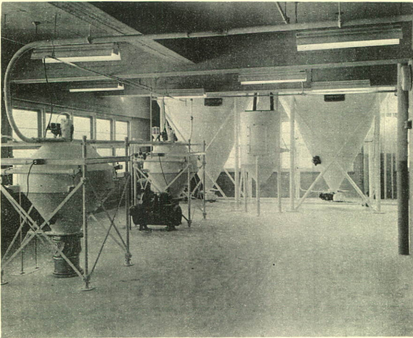
FLOUR BINS AND AUTOMATIC SCALES.
