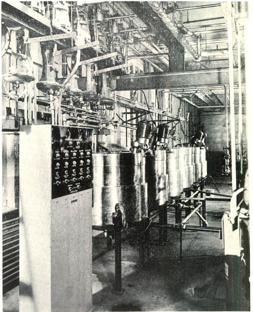
CONTROL PANEL AND SERIES OF BASINS FOR AUTOMATIC PREPARATION OF MARSHMALLOW.
