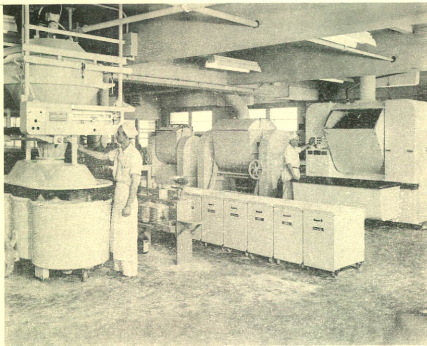
DOUGH PREPARATION DEPARTMENT: FLOUR' AUTOMATIC SCALE AND DOUGH MIXERS.
