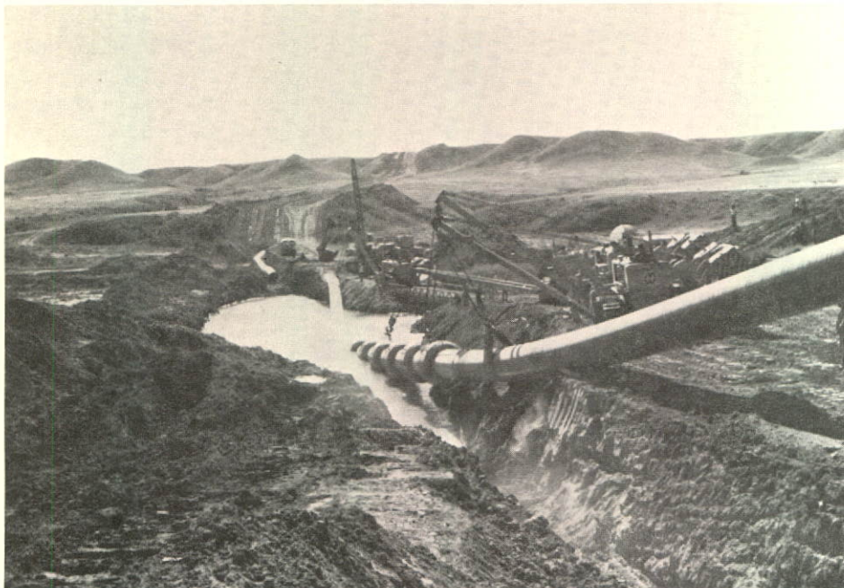
Sideboom tractors lower the pipe into the bed of the Frenchman River in southwestern Saskatchewan.
