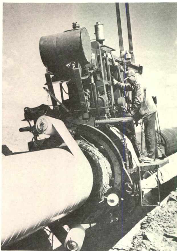
Wrapping operations at the pipeline crossing of the South Saskatchewan River in eastern Alberta.
