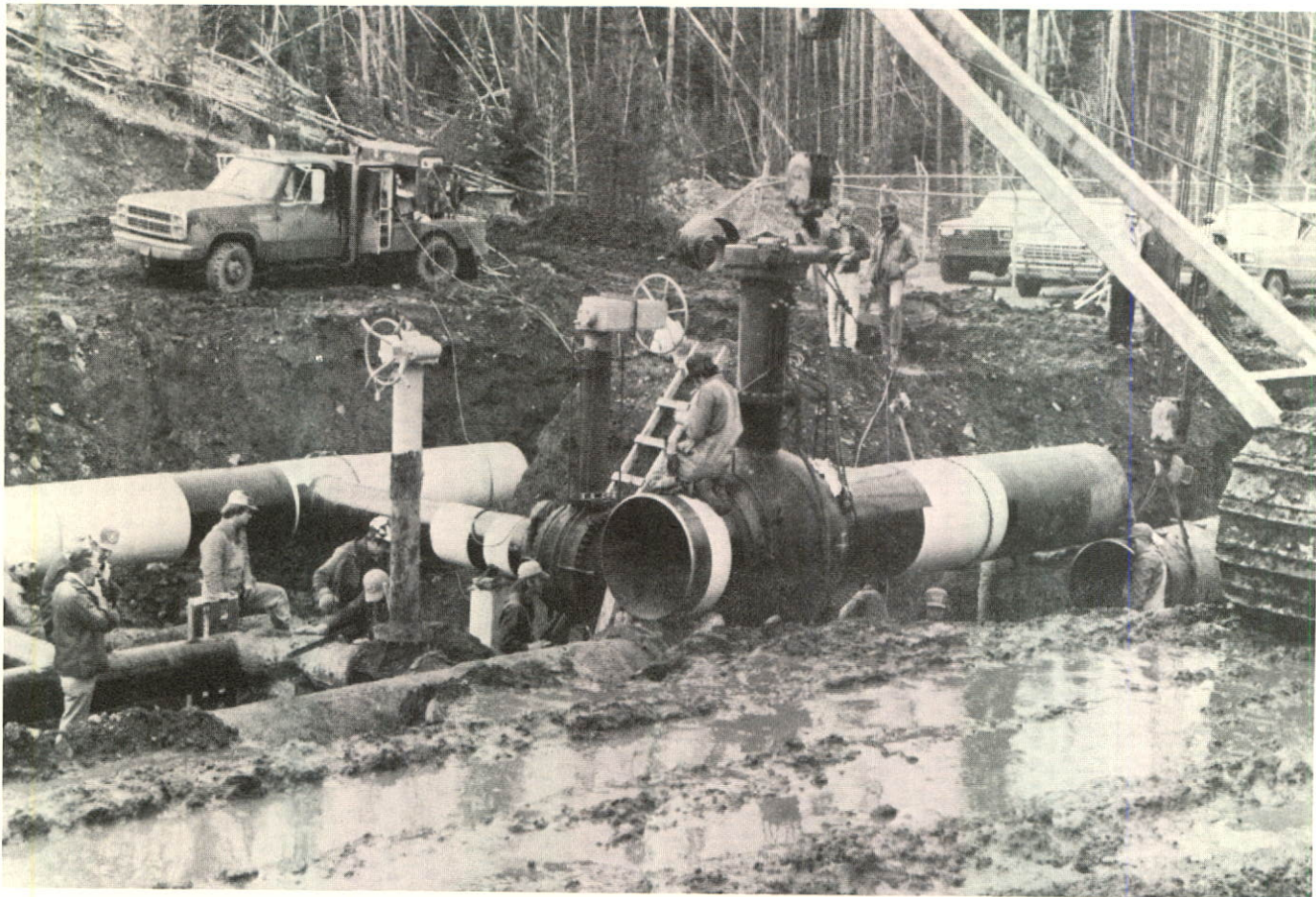
Final tie-in of the Western Leg into the system of Alberta Natural Gas Company Ltd. in the Crowsnest Pass area of southeastern B.C. in May 1981.
