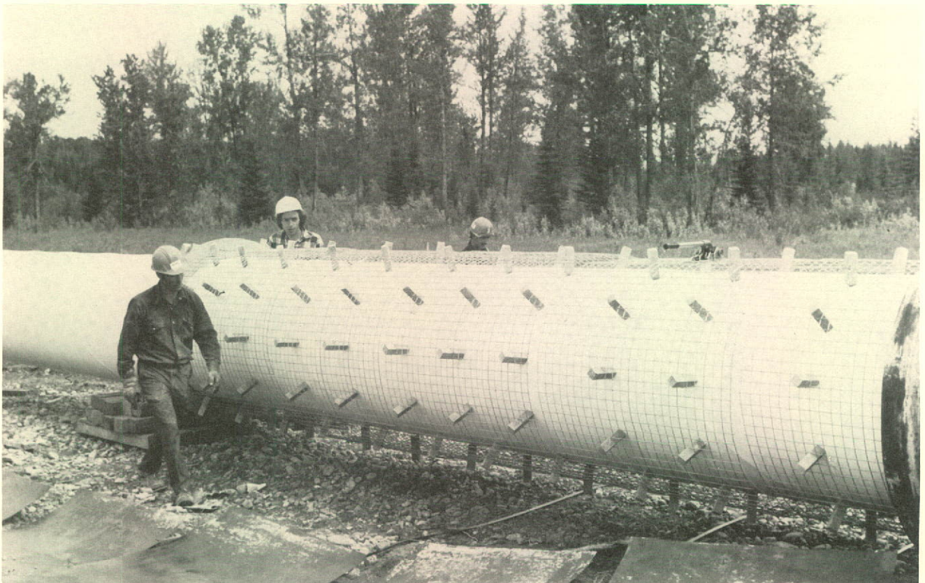
Construction crews wrap the pipe in wire mesh prior to its encasement in concrete.
