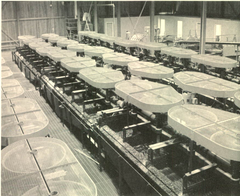
Flotation cells.
