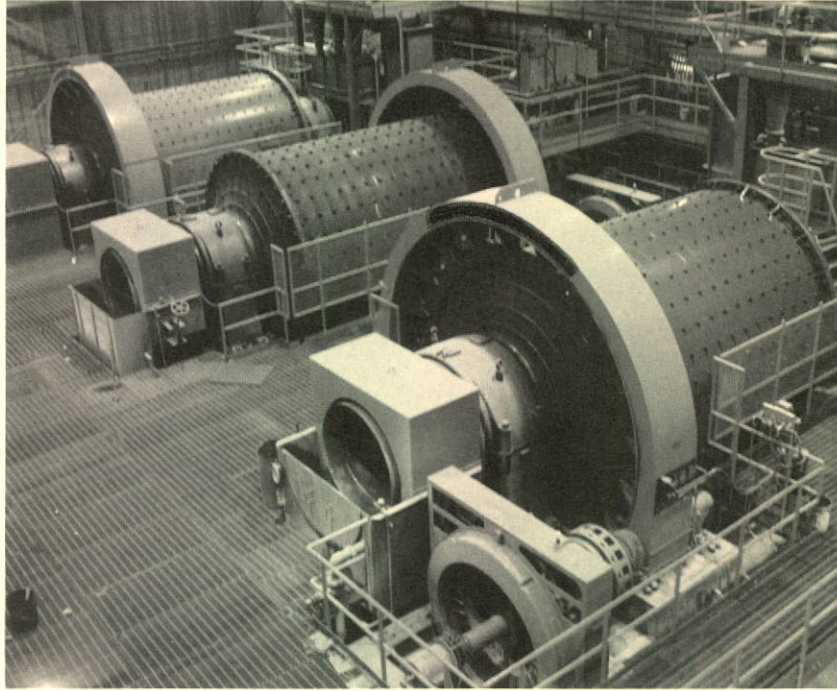
Grinding mills.
